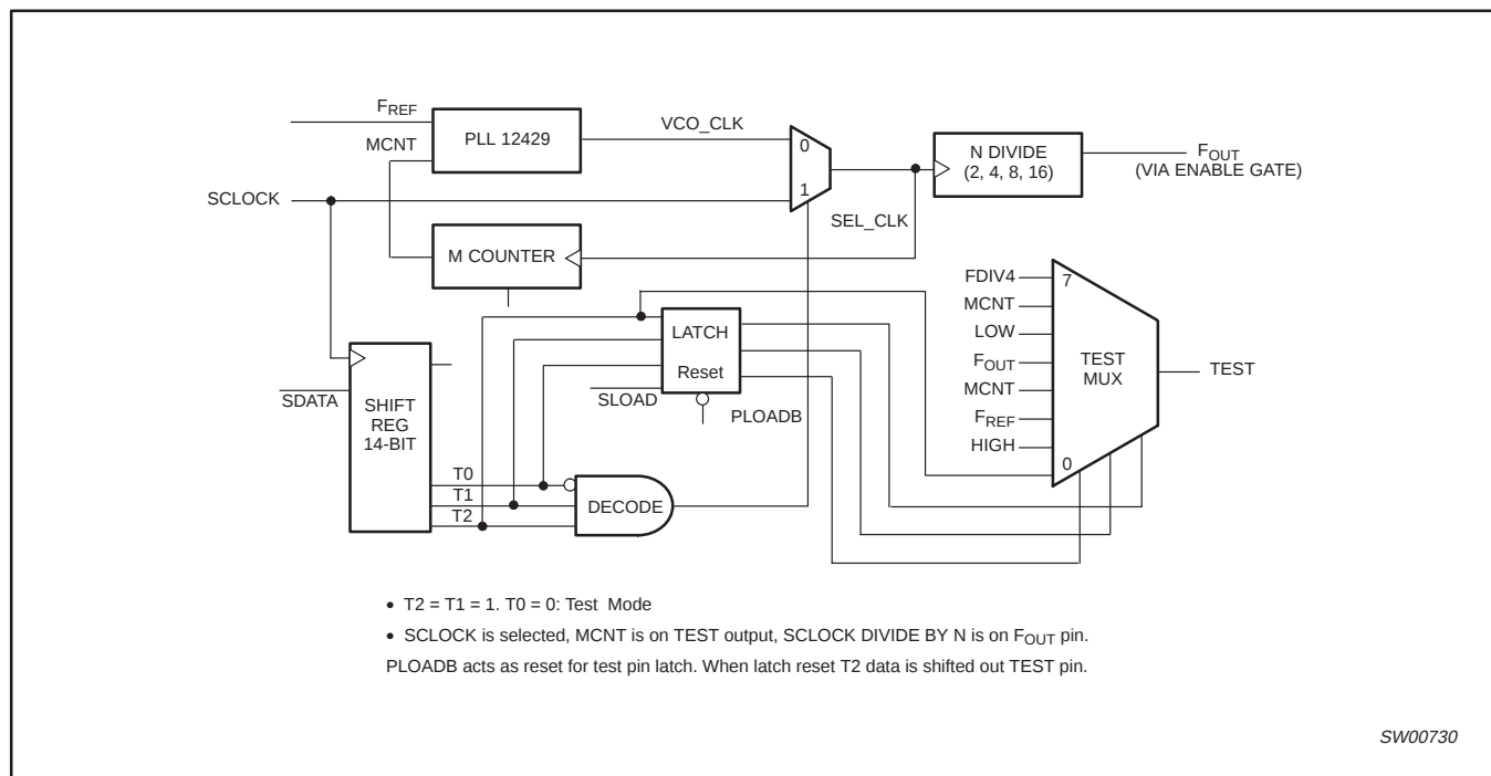
Figure 2. Serial Test Clock Block Diagram
