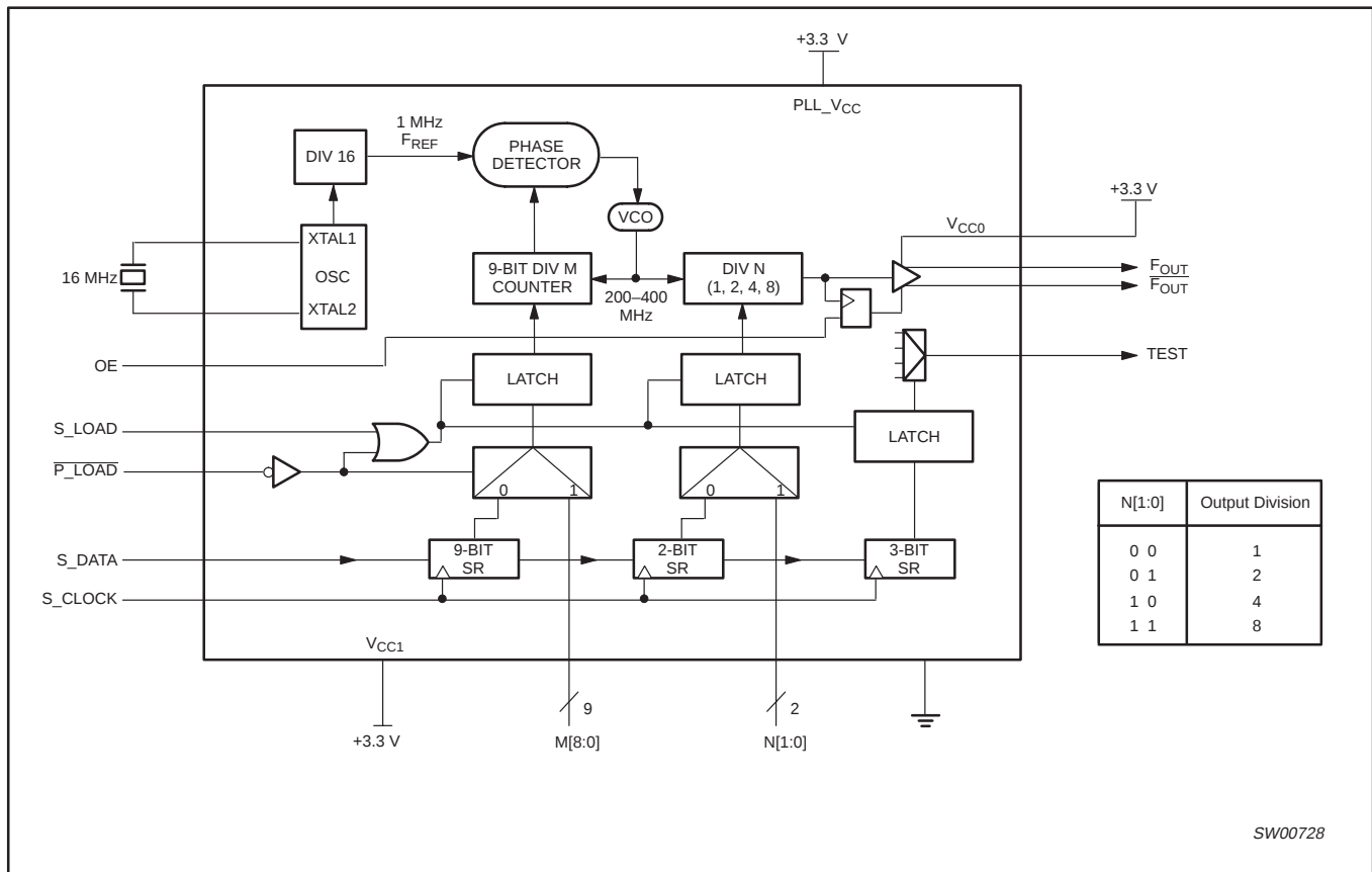
BLOCK DIAGRAM
